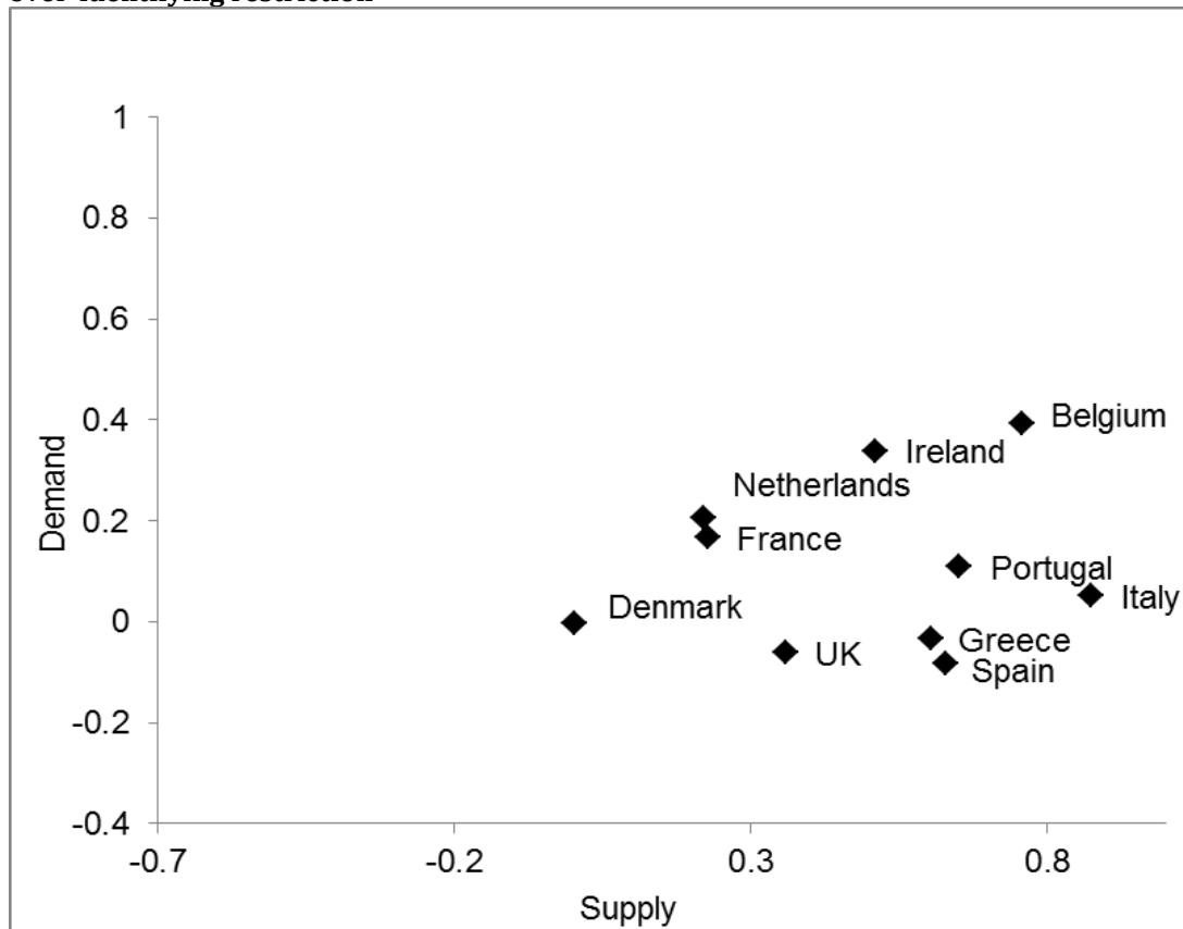
Figure 1A: Correlation of supply and demand disturbances vis-à-vis Germany imposing the over-identifying restriction
