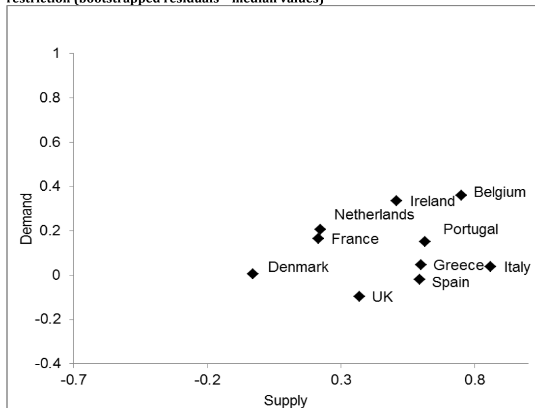
Figure 1: Correlation of supply and demand disturbances imposing the over-identifying restriction (bootstrapped residuals – median values)
