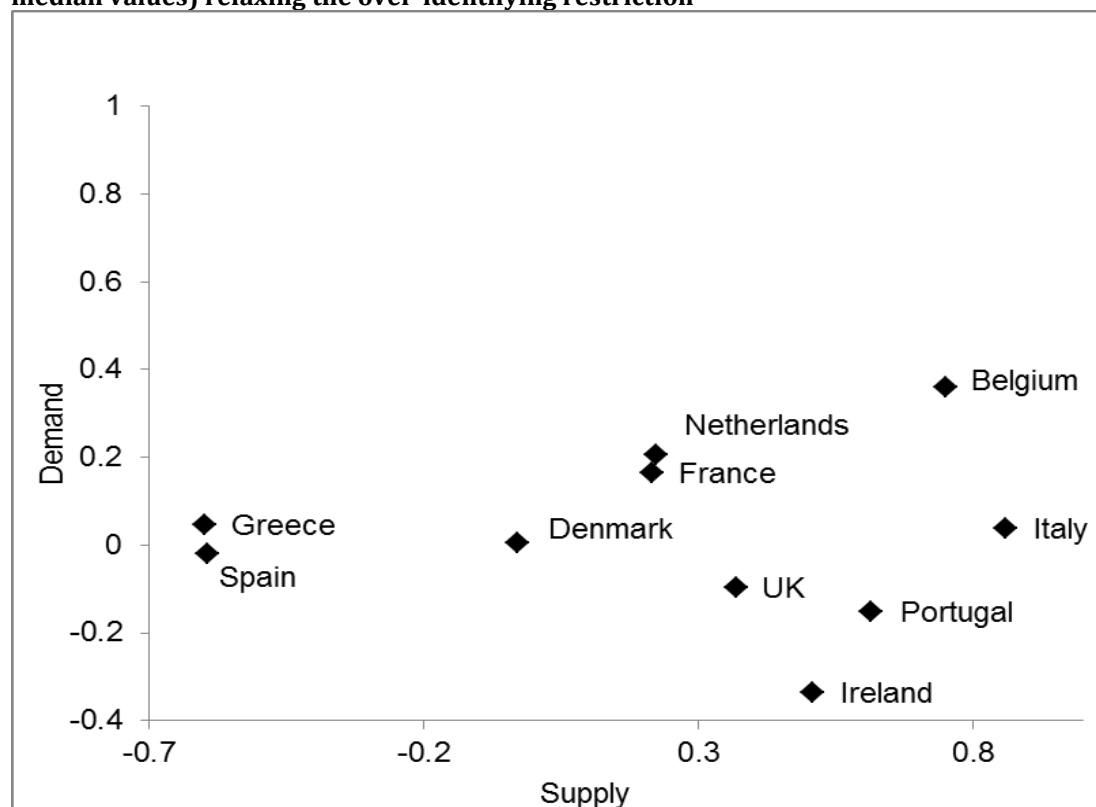
Figure 2: Correlation of supply and demand disturbances (bootstrapped residuals – median values) relaxing the over-identifying restriction
