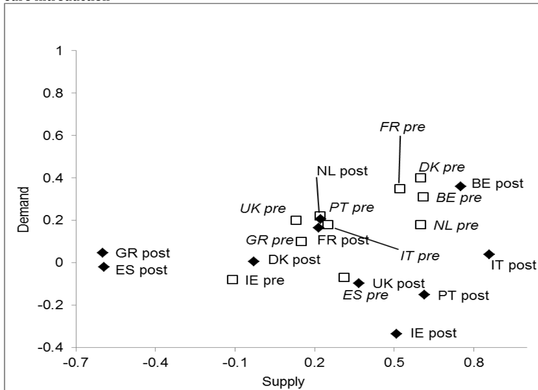
Figure 5A: Correlation of supply and demand disturbances vis-à-vis Germany, pre and post euro introduction
