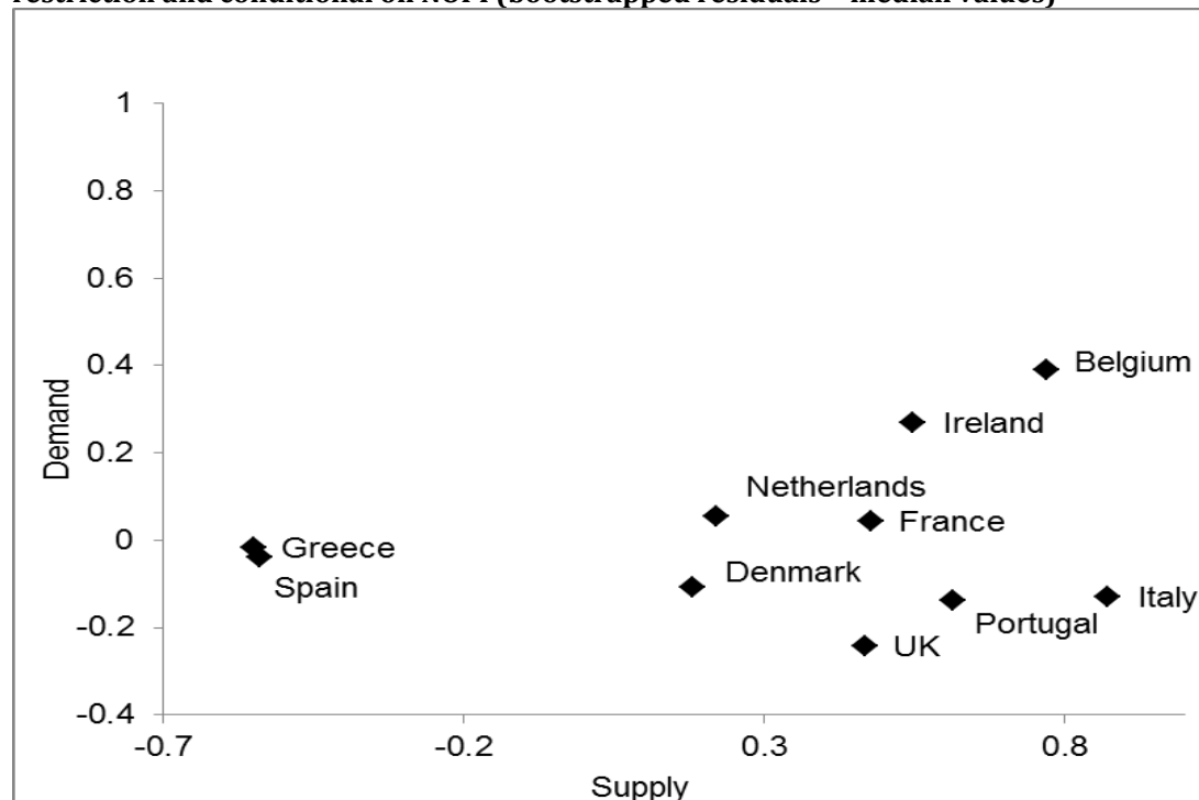
Figure 4: Correlation of supply and demand disturbances relaxing the over-identifying restriction and conditional on NOPI (bootstrapped residuals - median values)
