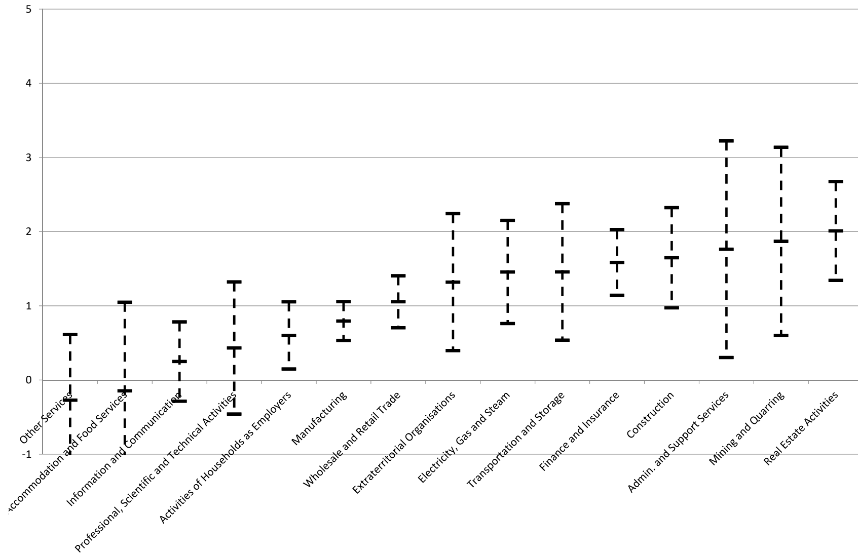
Figure 8: Sector Heterogeneity
