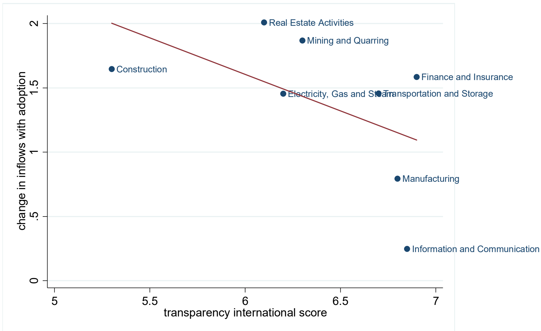
Figure 9: Sector Heterogeneity
