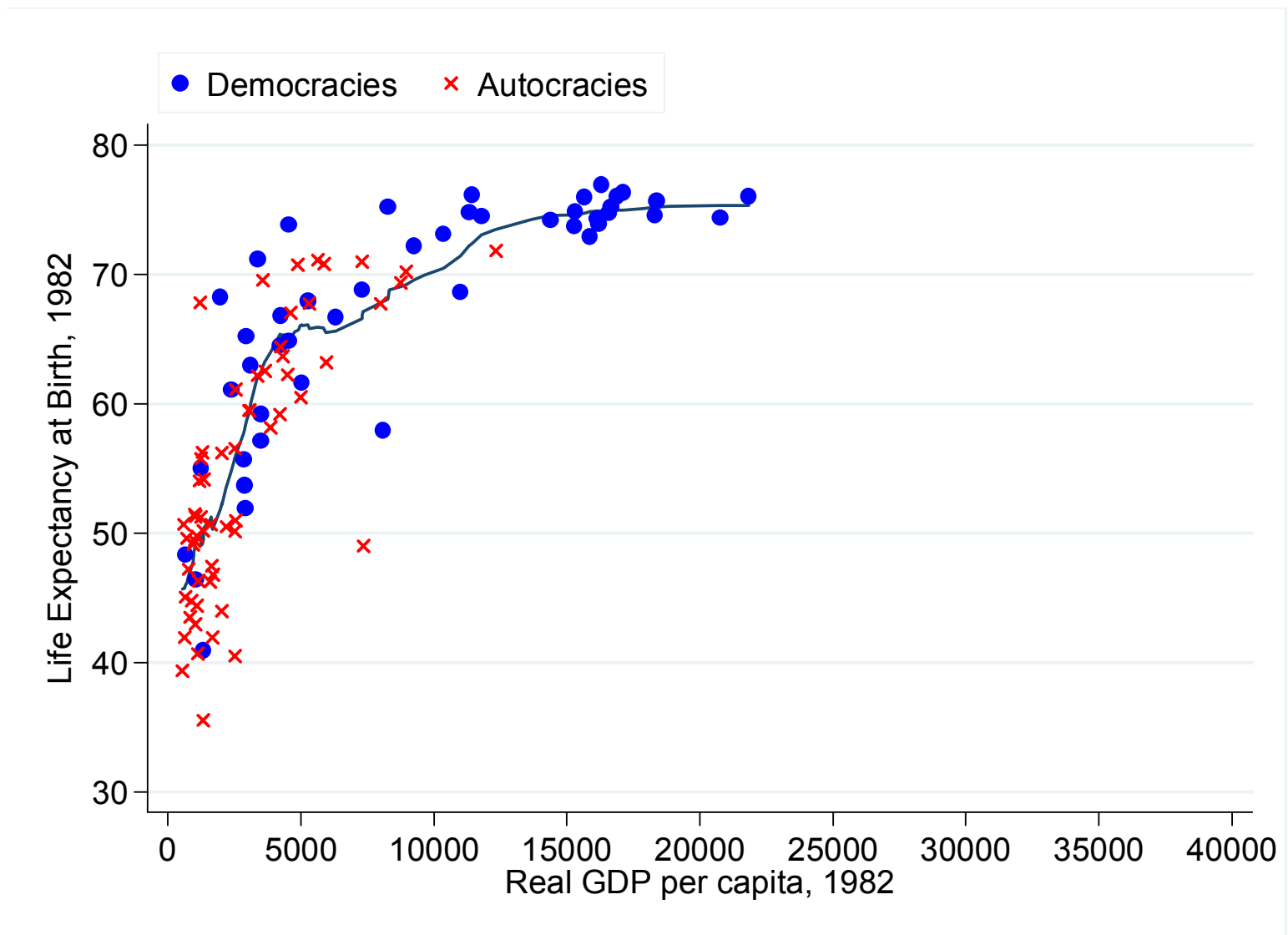
Figure 1: The Preston Curve in 1982
