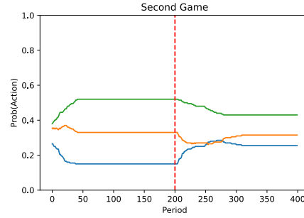
(b) Trust Collapse Effects Actions: Game 2
