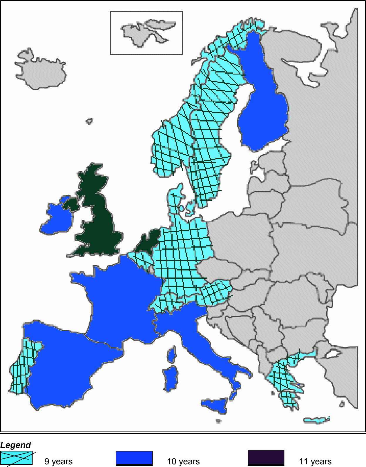
Figure 2 Number of years of compulsory schooling in 16 European countries, 2000
