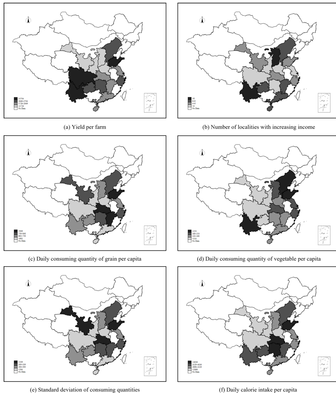
Figure 9. Area-level Variables
