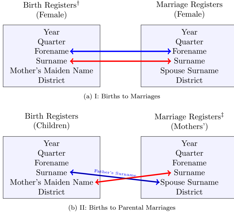
Figure 2.1: Linking Schema
