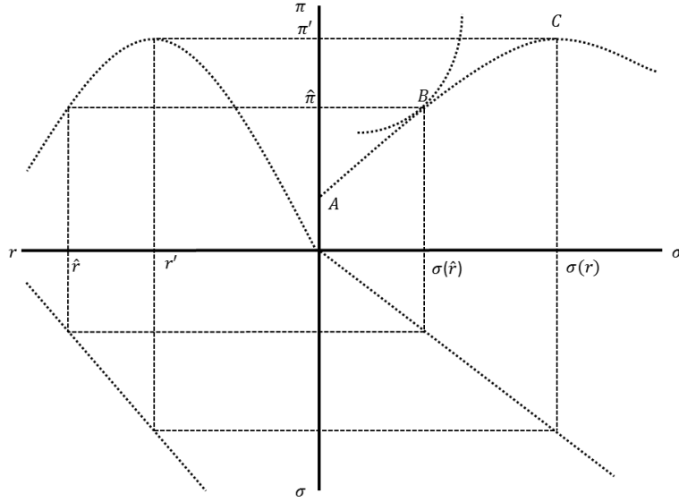
Figure 4: Bank Reserves, Risk and the Natural Rate
