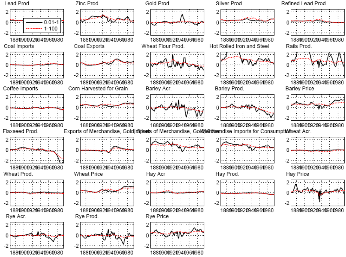
Figure 2: Factor Loadings, 1867-1995. Tight prior (red dotted line): \delta_{\epsilon} = 1, \alpha_{\epsilon} = 100 . Loose prior (black continuous line): \delta_{\epsilon} = 0.01, \alpha_{\epsilon} = 1 . Both priors imply the same mean of the IG distribution.
