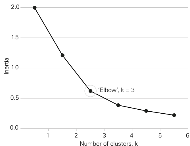
Figure 8: k-means Graph
