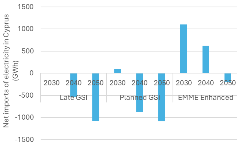
Figure 2. Volume of net imports of electricity in Cyprus in each scenario in the OSeMOSYS-Cyprus model (Late GSI, Planned GSI) and in the OSeMOSYS-EMME model (EMME Enhanced). Scenarios without interconnection are not shown, as no electricity can be traded.
