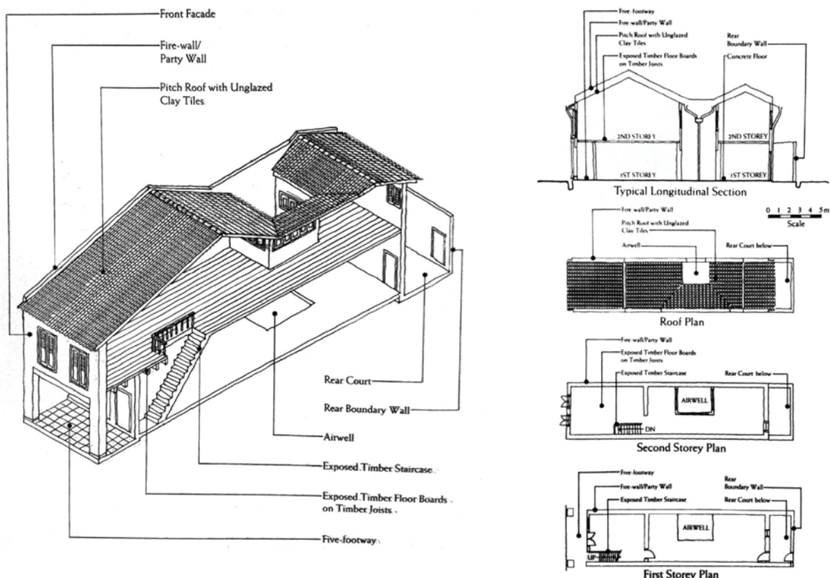
Figure 55: Spatial analysis of a typical shop house (Source: Urban Redevelopment Authority, 1995)
