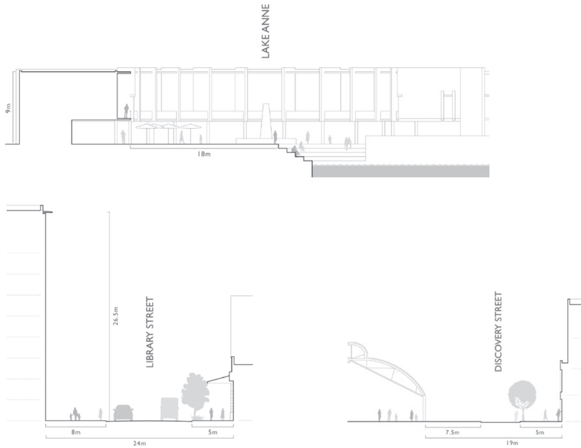
Figure 45: Diagram illustrating comparative street sections
