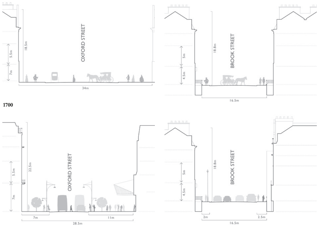
Figure 8: Diagram illustrating comparative street sections
