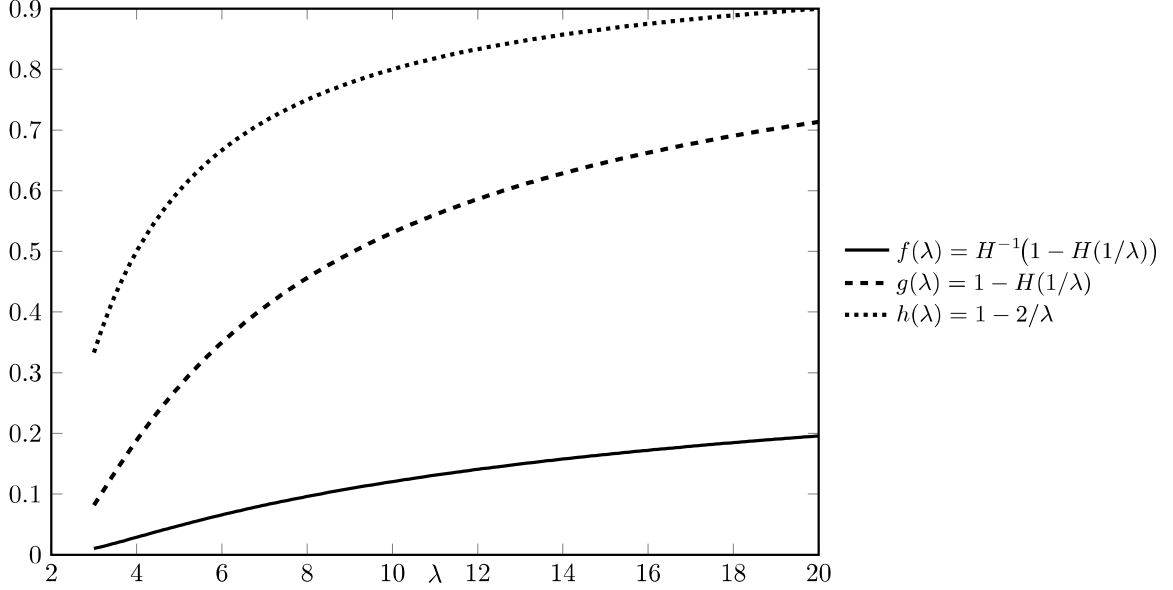
Figure 1: Graphs of f, g, h (from bottom to top) over the domain [3, 20] .
