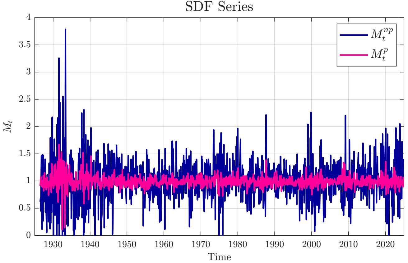
Figure 3: Estimated SDFs
