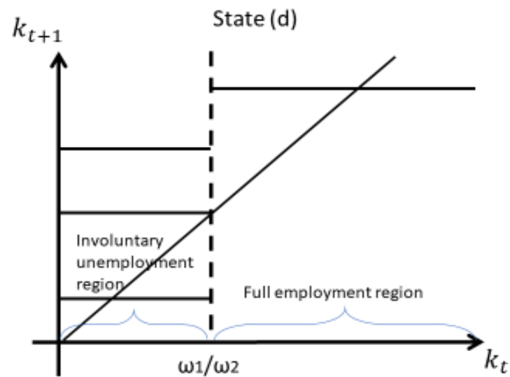
Figure 5-1: Wobbly macro-dynamics in the Leontief case
