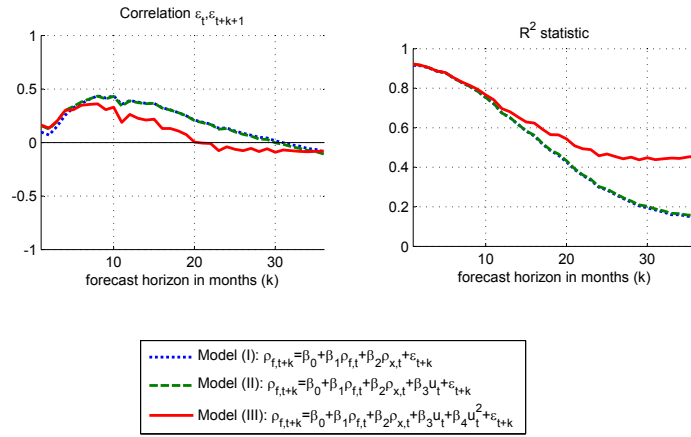
Figure A9: Diagnostics statistics: OLS estimator
