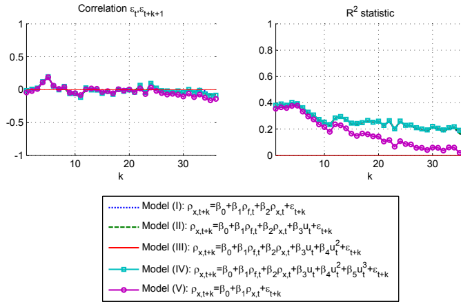
Figure A13: Diagnostics statistics: job loss rate
