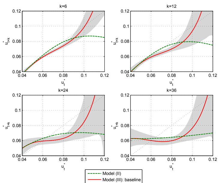
Figure A6: Steady states: duration-based CPS data (1970-2015)
