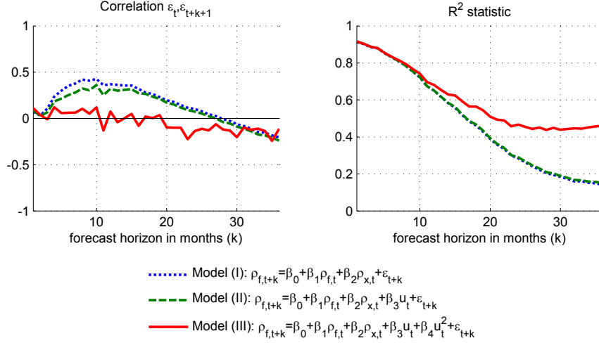
Figure 3: Diagnostic statistics.
