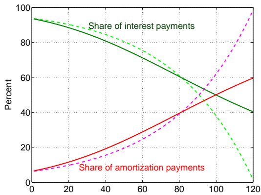
Figure A.1: Mortgage loan: model (with \kappa = 0.00162 and \alpha = 0.9946 ) v.s. real-world mortgage (Yahoo mortgage calculator). Solid line=model, dashed line=real-world mortgage. Here, l_0 = \$250,000 and i = 9.28\%/4 . The approximation error is expressed as the present value (using 1/i ) of the difference between the installments in the model and in the mortgage calculator, divided by the size of the loan.
