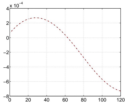
Figure A.1: Mortgage loan: model (with \kappa = 0.00162 and \alpha = 0.9946 ) v.s. real-world mortgage (Yahoo mortgage calculator). Solid line=model, dashed line=real-world mortgage. Here, l_0 = \$250,000 and i = 9.28\%/4 . The approximation error is expressed as the present value (using 1/i ) of the difference between the installments in the model and in the mortgage calculator, divided by the size of the loan.
