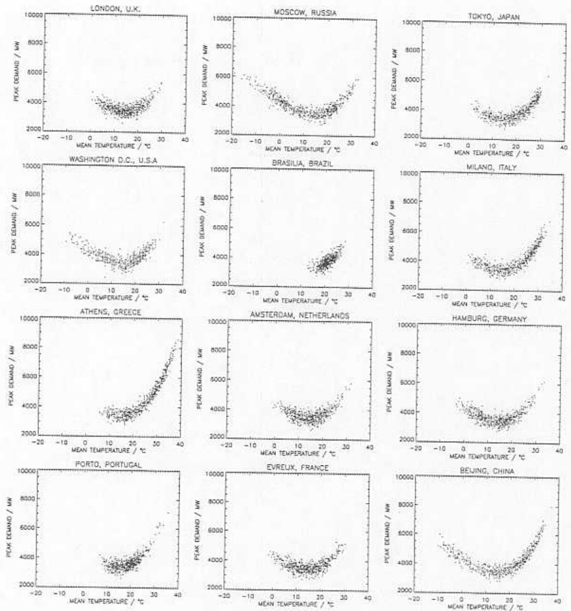
Figure 19: Synthetic demand plotted against temperature for the 12 locations used in the experiment. The temperature-demand relationship used is given by Eq. 7.
