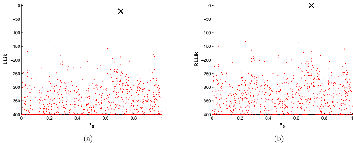
Figure 1. Typical log-likelihood of 1024 states (uniformly distributed on [0, 1] ) for the logistic map. The true initial condition \tilde{x}_0 = \sqrt{2}/2 (denoted by “ \times ”), \sigma = 0.1 , and n = 32 . (a) Log-likelihood function, (b) relative log-likelihood to \tilde{x}_0 . States which have (relative) log-likelihood less than -400 are plotted on the -400 horizontal line. All logarithms are using the natural base. The maximum likelihood value found was \sim e^{-109} , which corresponds to log-likelihood of -132 relative to Truth.
