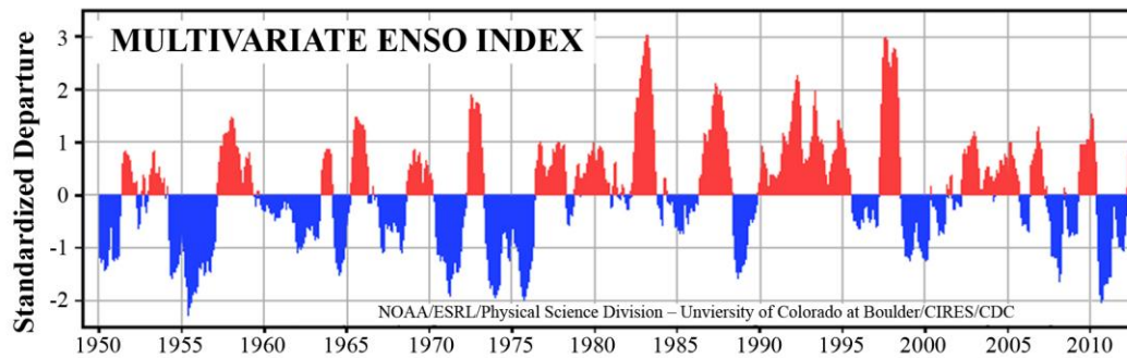
Figure 13. ENSO Index.
