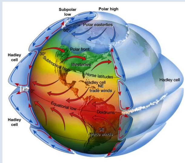
Figure 30. Atmospheric Circulation.
